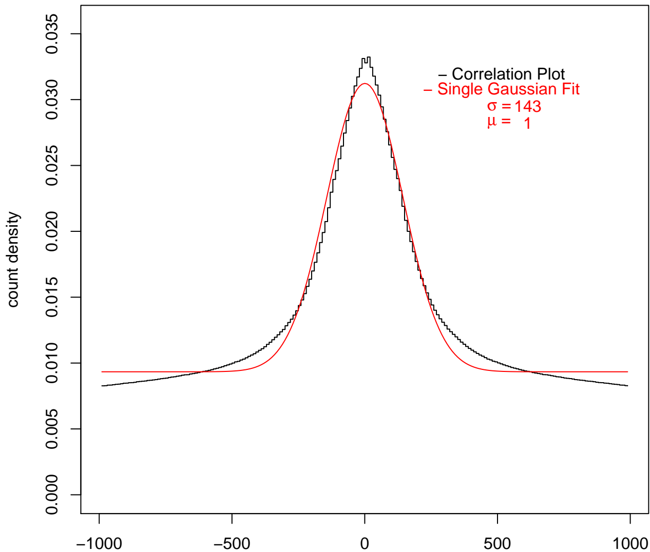
Positional relationship between STAT1-stim (75 bp centered) and STAT1-stim (75 bp centered)
